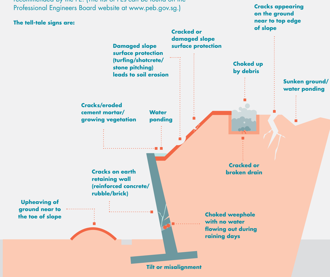
Cross section showing various tell-tale signs of slope failure
